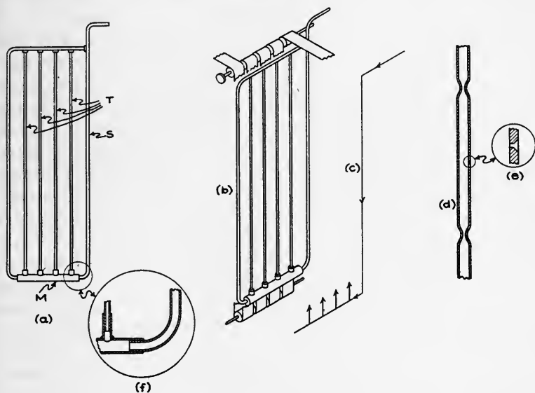
FIG. 3. Details of vertical grid distributor: (a) distributor, (b) position of distributor relative to rack, (c) path of air through distributor, (d) method of introducing additional resistance to flow of air in oversized distributor tubes, (e) orifice in distributor tube, (f) construction details of distributor manifold.
